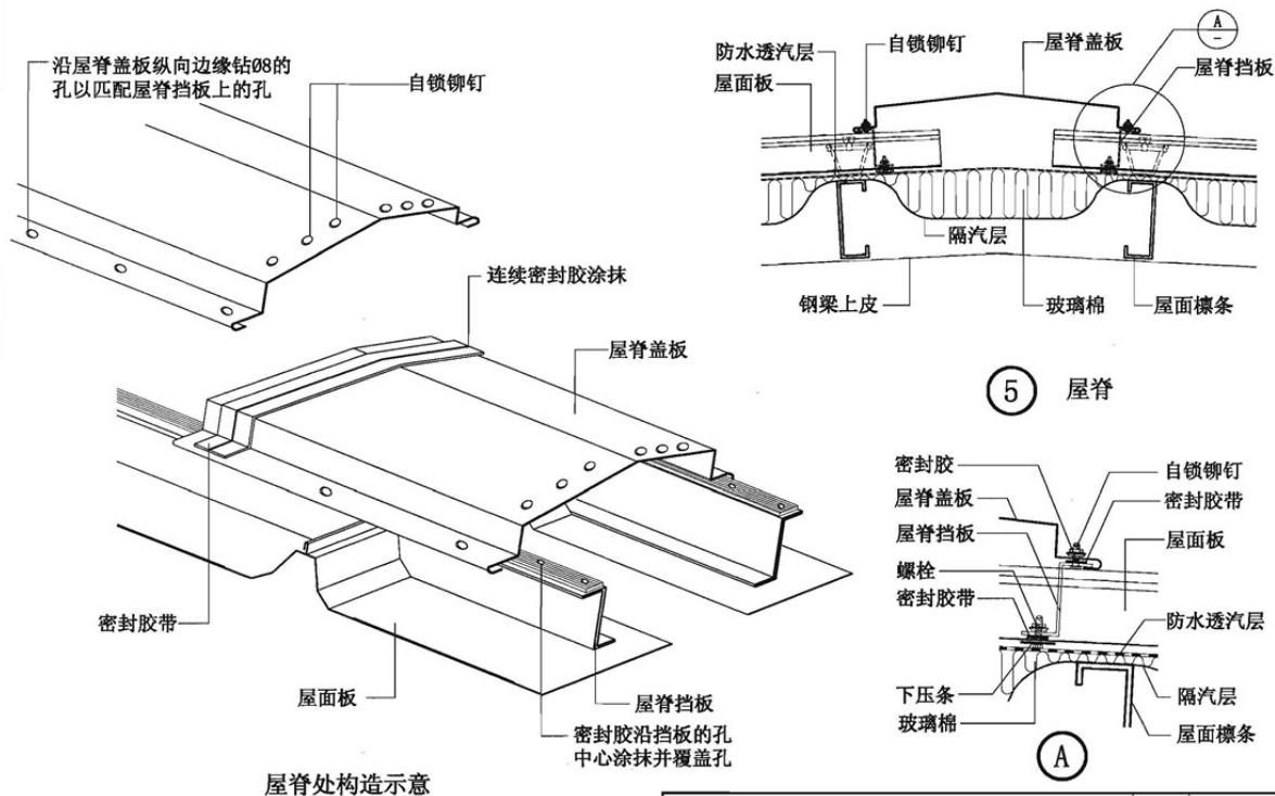
压型钢板复合保温直立缝滑动屋面双坡屋脊
