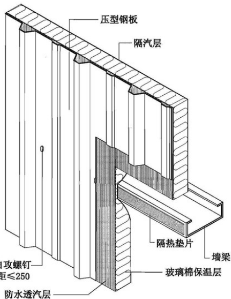
墙2A-单层压型钢板复合保温墙体(竖向排板)构造
